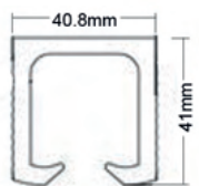
7200 Heavy Duty Aluminium Track 510-3001-200
