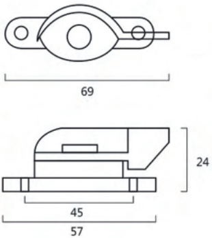
CF350 Crescent Fastener (NA)-L
