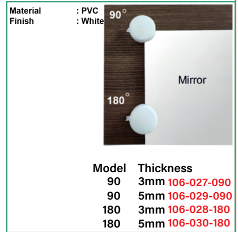
Glass Clip
