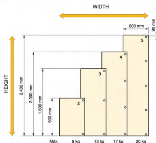
NUMBER OF HINGES NEEDED FOR EACH DOOR
