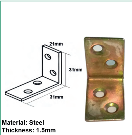
21x31x31 L-Bracket
