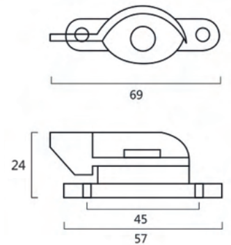
CF350 Crescent Fastener (NA)-R
