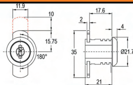
3502U-01-G491 Desk Drawer Bolt Lock
