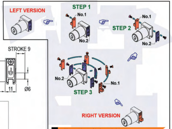
Illustration of left or right side installation for 3642 series
