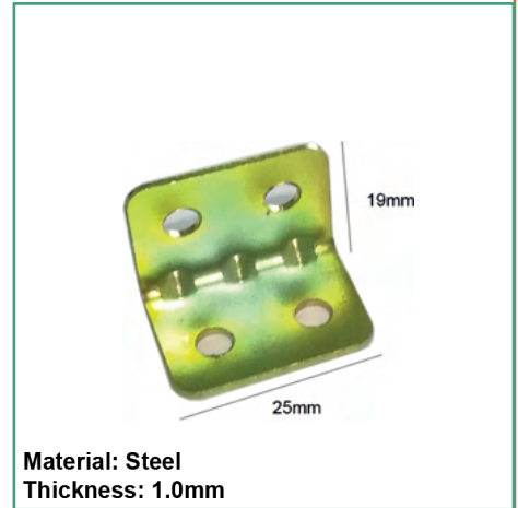
3/4" RB L-Bracket
