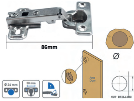
260 CSS Hinges (S) 500-110-260
