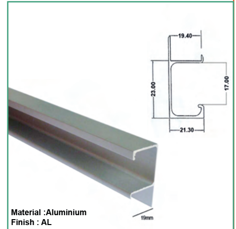
1923 Aluminium Handle 12ft
