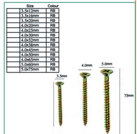
Chipboard Screw
