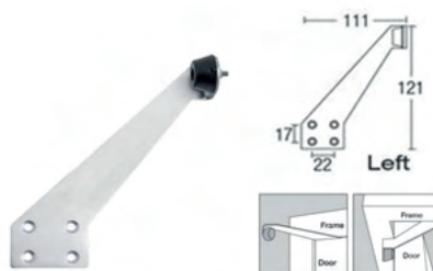
Material: Stainless Steel Finishing: SN J7 Wall Mount Door Stopper (L) StG-WMDS-SS
