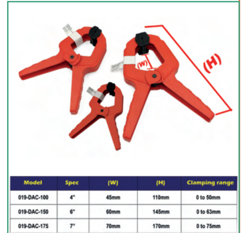
Duratec A-Clamp
