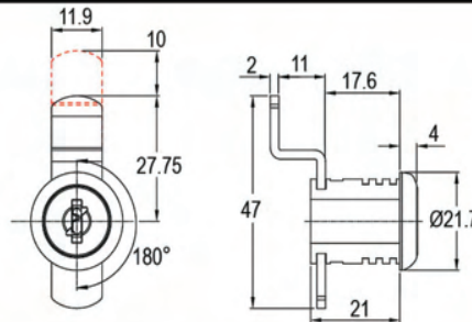
3502U-01-G490 Desk Drawer Bolt Lock
