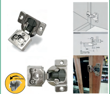
TS70 Hinge With Soft Closing 500-TS-70
